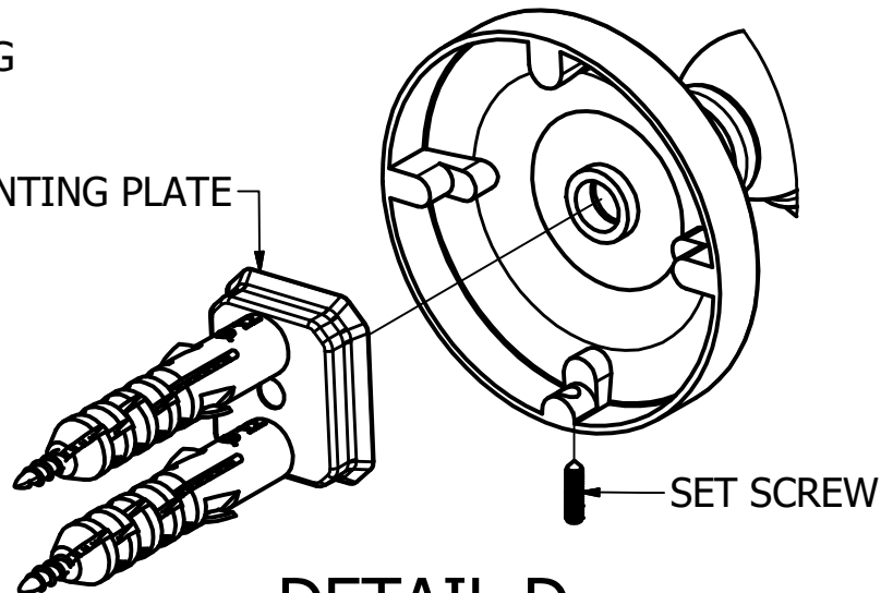
DETAIL D
